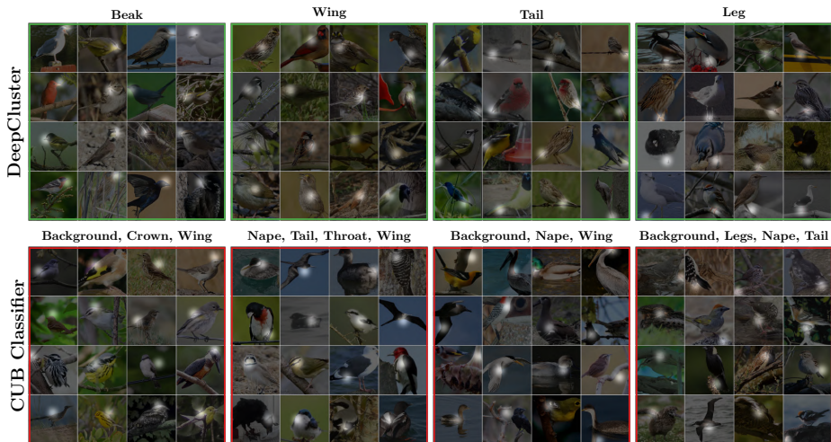
Fig. S1: Clustering visualizations. We study part disentanglement when clustering the spatial features obtained with different auxiliary models. We highlight image regions assigned to the same cluster (best viewed in color digitally). We indicate the parts found in each cluster for the purpose of visualization.
