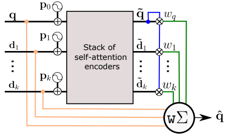
Fig. 2. Proposed aggregator. The output \hat{\mathbf{q}} is constructed as the weighted sum ( \bar{\mathbf{w}}\Sigma ) of the query \mathbf{q} and the nearest neighbors \mathbf{d}_1 \dots \mathbf{d}_k . The weights are computed by running the inputs through a stack of self-attention encoders after including positional information ( \oplus ) and computing the similarity (through a normalized dot product \otimes ) between the transformed query \tilde{\mathbf{q}} and all the transformed samples \tilde{\mathbf{d}}_1 \dots \tilde{\mathbf{d}}_k .
